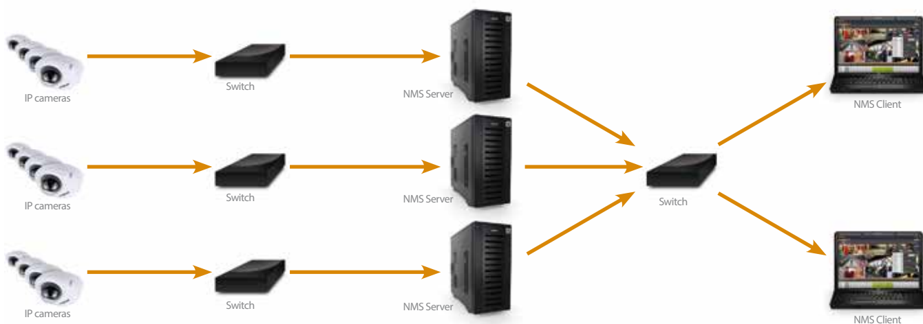
Complex system based on specialized workstations – NMS Server and NMS Client
